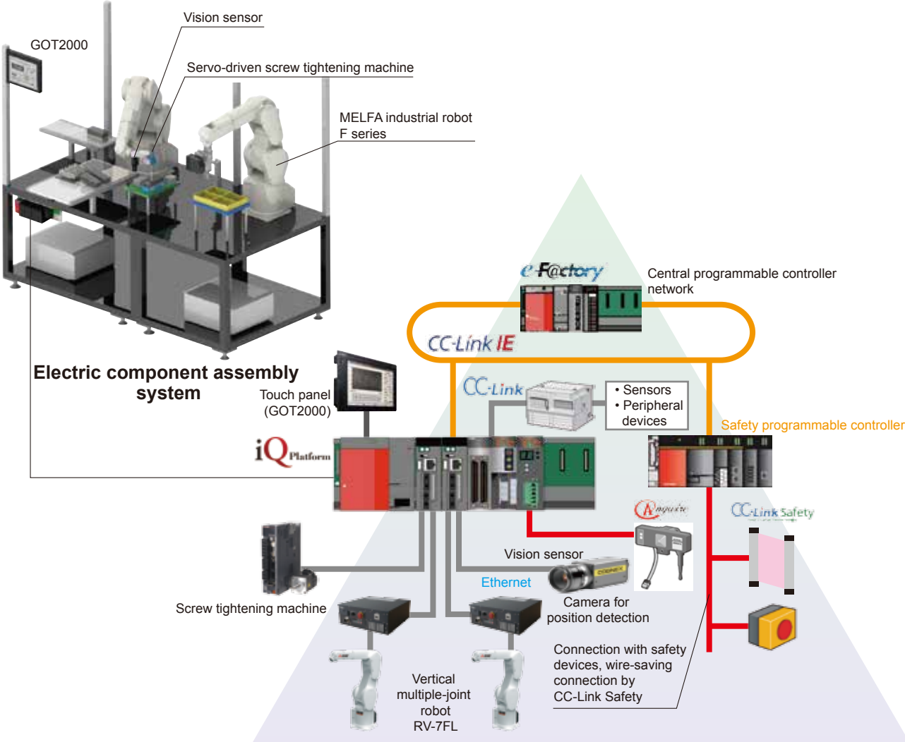
Control device configuration
