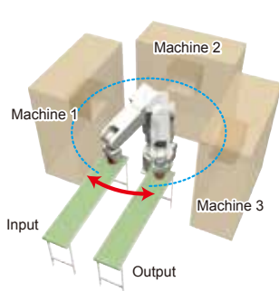
RV-2FQ/2FD pivot operation
