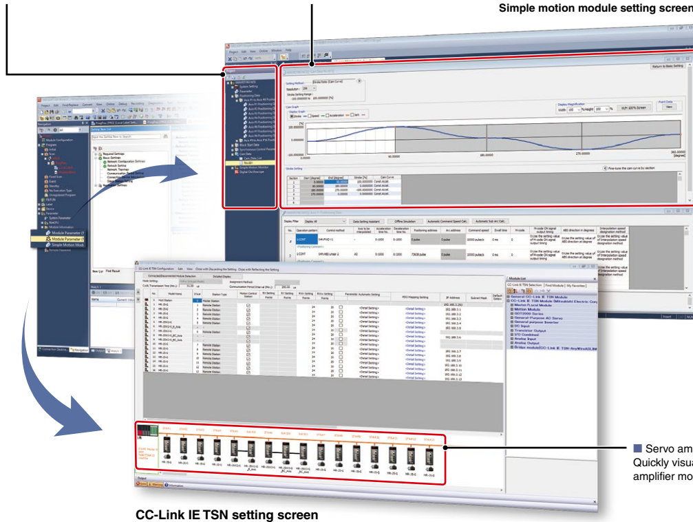
CC-Link IE TSN setting screen
